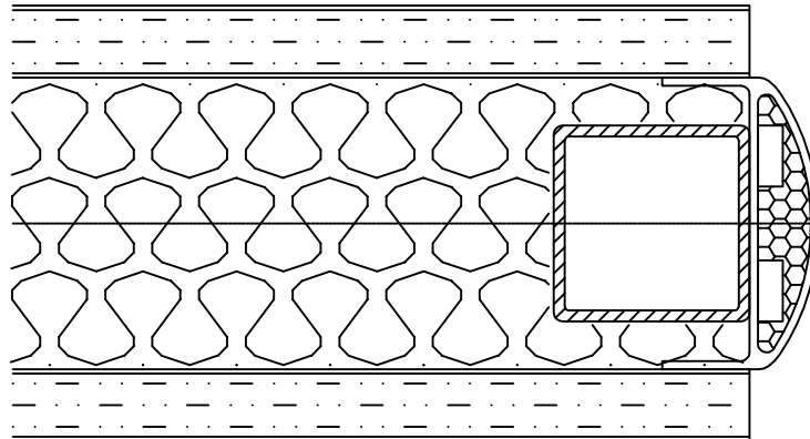
PLAN SECTION at WALL ABUTMENT WDE (Bulb Seal)
