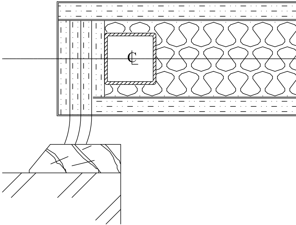
PLAN SECTION at WALL ABUTMENT with LIPSEAL
