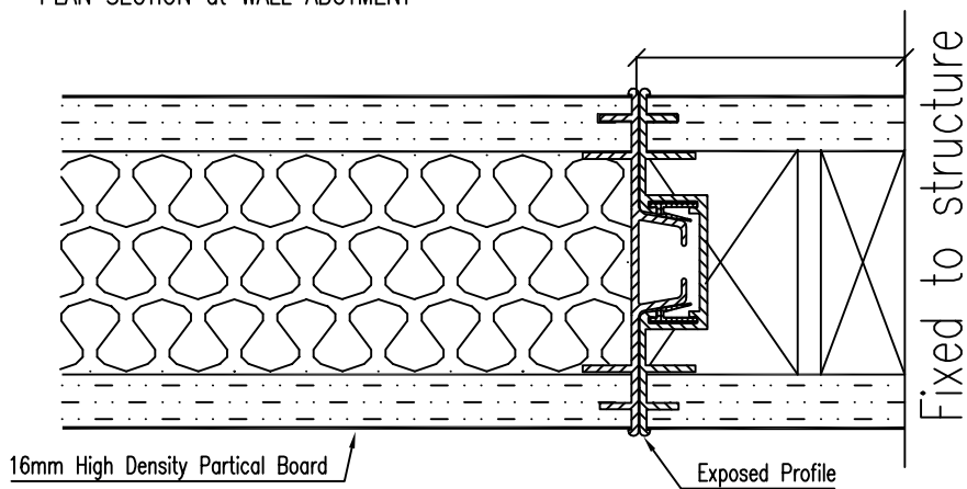
PLAN SECTION at WALL ABUTMENT
