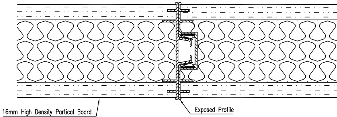
PLAN SECTION at PANEL JOINT
